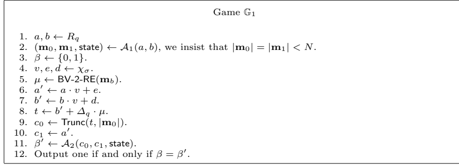
Figure 6. Game \mathbb{G}_1
