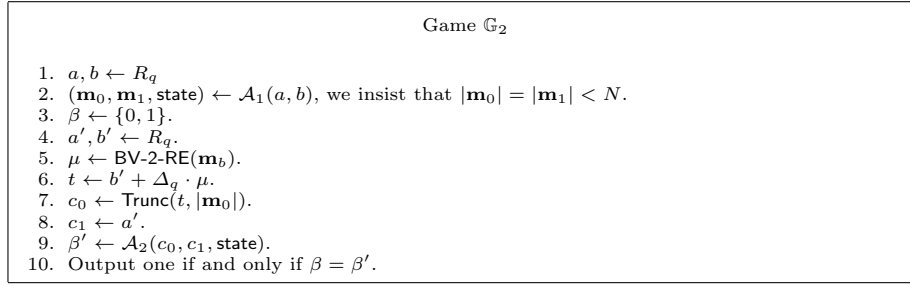
Figure 7. Game \mathbb{G}_2
