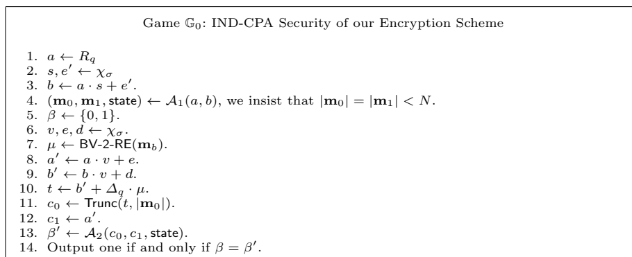
Figure 5. Game \mathbb{G}_0 : IND-CPA Security of our Encryption Scheme
