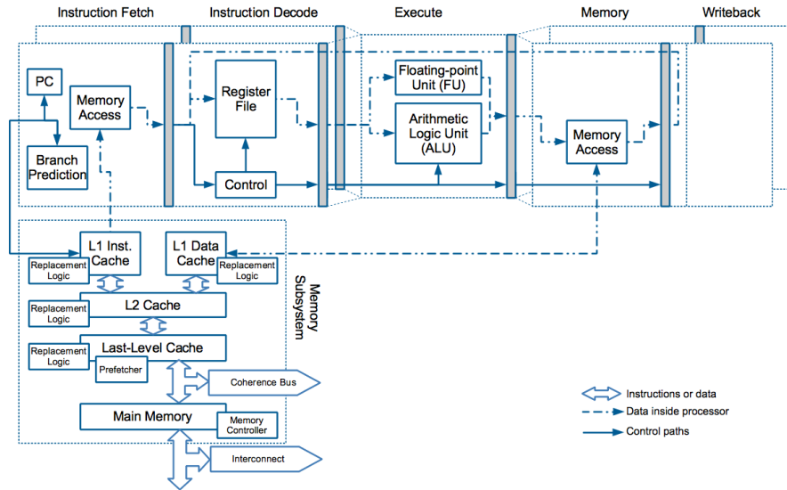
Fig. 1: The prototypical two-thread SMT processor with 5-stage processor pipelines shown with shared execution stage and key components of the memory subsystem.
