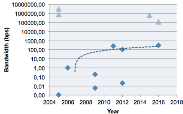
Fig. 6: Scatter plot of attacks from Table 1 along with a trend line showing roughly 10x improvement in attack bandwidth over last 10 years for the non-idealized attacks (squares). Idealized attacks (triangles) show much greater bandwidth, but these are for specific cases, such as attacks on particular table lookup based AES software implementation or particular RSA implementation
