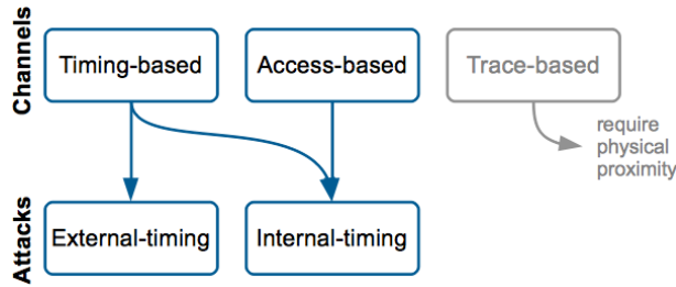
Fig. 5: Relation between channel types and attack types.
