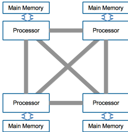
Fig. 4: Example of 4-processor setup with point-to-point (QPI-like) interconnect between them. Each processor has its own associated memory, but all processors can access the other memories via the interconnect, a typical NUMA configuration for systems with a single global address space.
