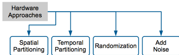
Fig. 8: Main hardware approaches to microarchitectural side and covert channel defense.
