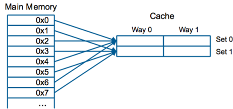
Fig. 2: Example of a two-way set-associative cache. Data from each memory location is assigned to a specific set, based on the address. Multiple ways allow storing multiple pieces of data in a same set. The LRU policy is used within each set.
