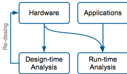
Fig. 7: Design-time analysis takes into account the hardware properties. Run-time approaches can combine both hardware and software properties, but are done post-design and are not able to influence the re-design of hardware, which could minimize the side and covert channel capacities.
