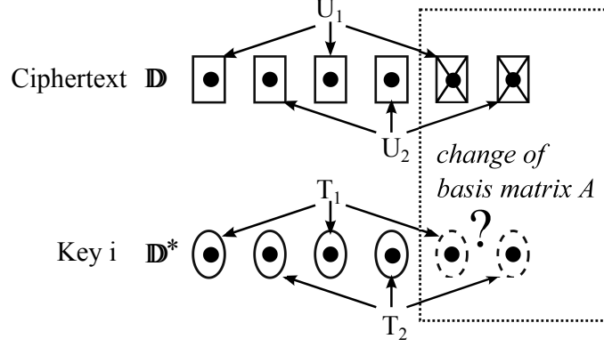
Figure 5: Key i expands into semi-functional space
