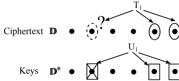
Figure 6: The coefficient of \vec{d}_2 in the ciphertext is randomized
