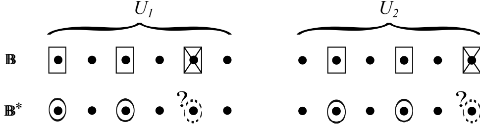
Figure 2: Subspace Assumption with k = 2
