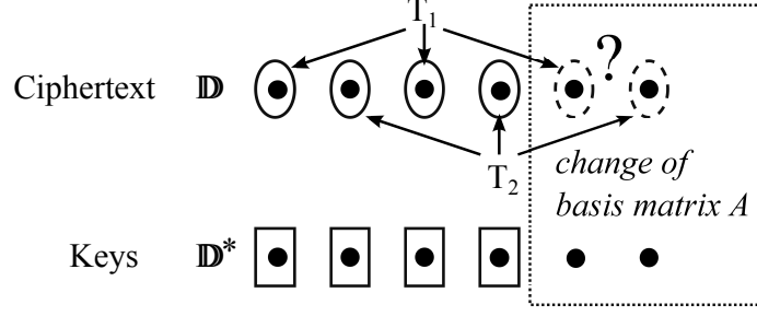
Figure 4: Ciphertext expands into semi-functional space
