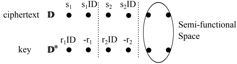
Figure 3: Cancellation in our construction
