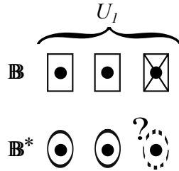
Figure 1: Subspace Assumption with k = 1
