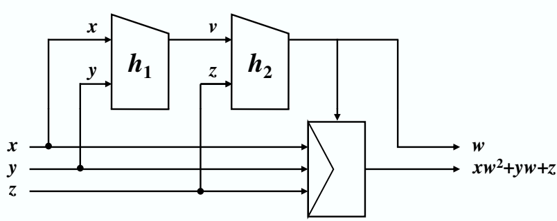
Fig. 7. The quadratic cascade compression function.
