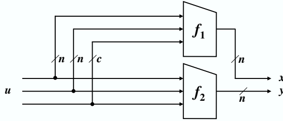
Fig. 8. Lucks' double-piped compression function
