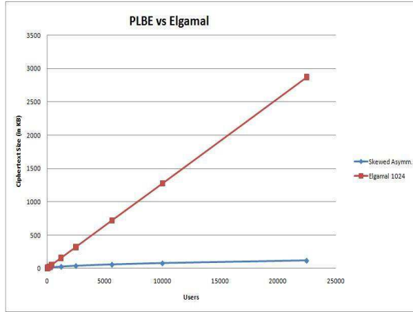
Fig. 5. Ciphertext Size
