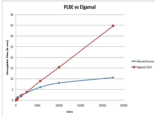
Fig. 6. Encryption Time
