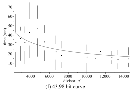
Fig. 5: Quartile plots of the running times for Cheon's algorithm.
