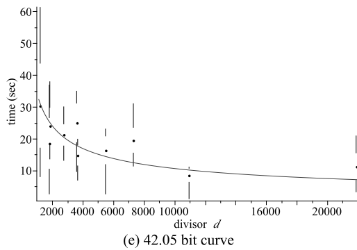
Fig. 5: Quartile plots of the running times for Cheon's algorithm.
