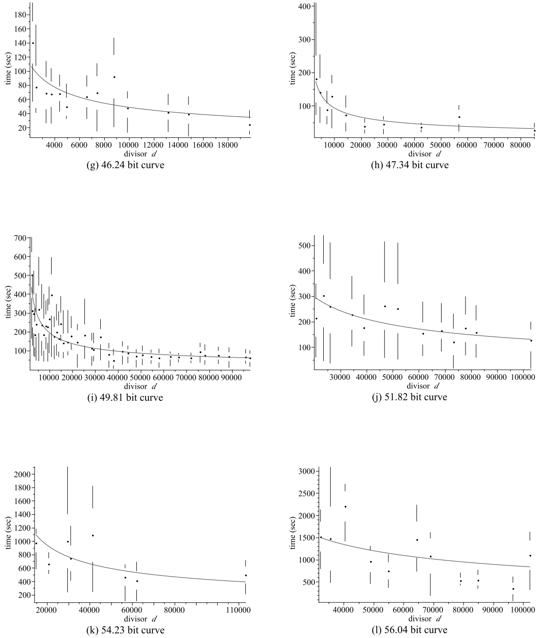
Fig. 5: Quartile plots of the running times for the Cheon's algorithm (continued).
