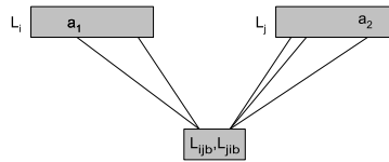
Fig. 1. Precomputation.
