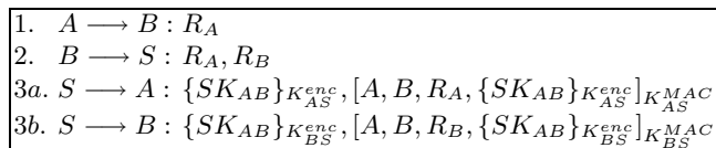
Fig. 5. Bellare–Rogaway 3PKD protocol
