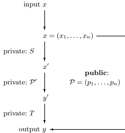
Fig. 2. \mathcal{MQ} -trapdoor (S, P', T) in STS
