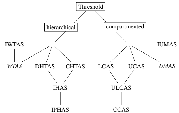
Fig. 1. A Taxonomy of Ideal Multipartite Access Structures
