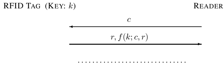
Figure 1: A generic challenge-response RFID protocol.
