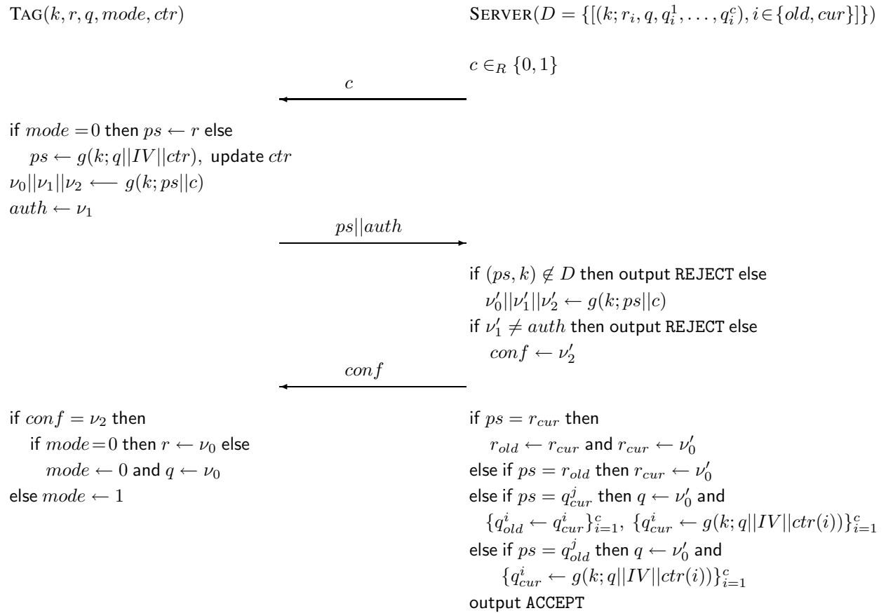
Figure 2: An anonymous RFID authentication protocol that supports constant key-lookup.
